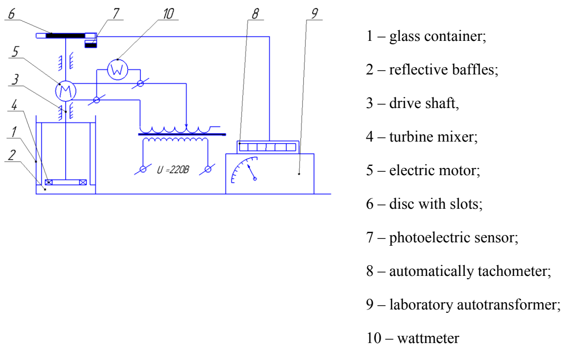
Figure 1 – Experimental installation
